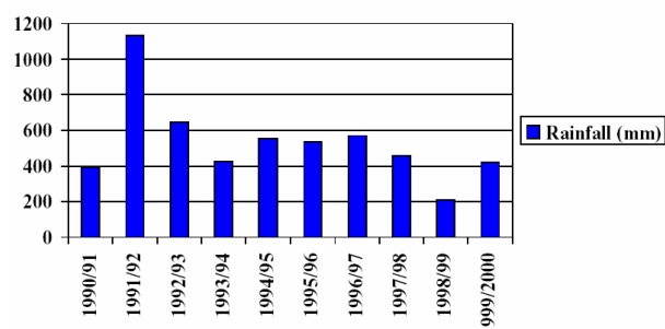
Figure 2-1 10-year cycle of rainfall in Israel xxii .
